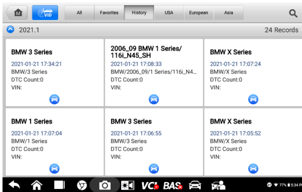
Figure 4-24 Sample History Screen
